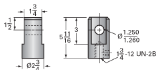
Clevis End (optional): 9001-SS-06
