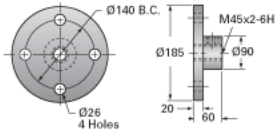
Top Plate (optional): 9000-EM-06
