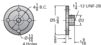
Top Plate (optional): 9000-00-03
