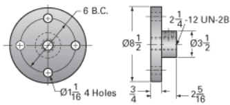
Top Plate (optional): 9000-00-07
